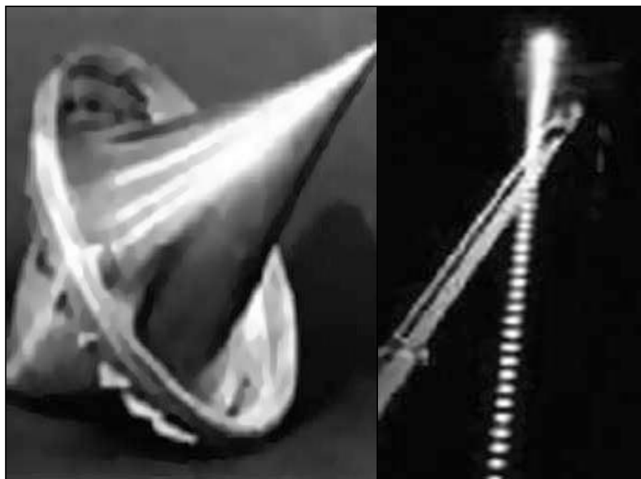
Figure 3.3.2. Launch of vehicle (SC) by low rate P-P laser (Rep. rate -20Hz, P=10kW).
