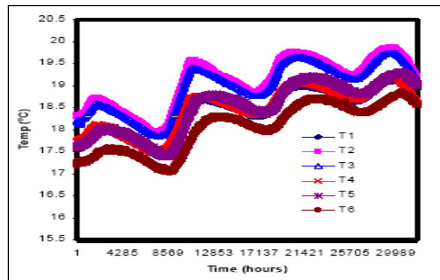
Figure 19. Variation of temperatures for heat exchanger for year
