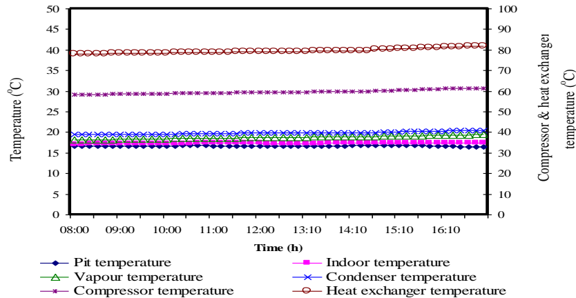
Figure 5. Variation of temperatures per day for the DX system
