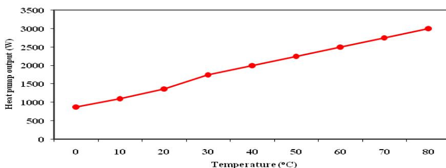
Figure 20. Variation of heat pump output with temperature
