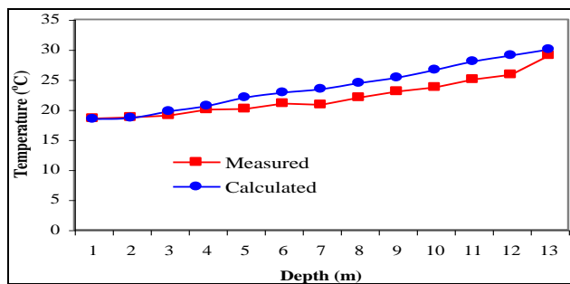
Figure 10. Comparison of calculations and experiments for saturated soil with groundwater flow (SSG)
