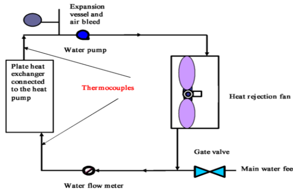
Figure 1. Sketch of installing a heat pump
