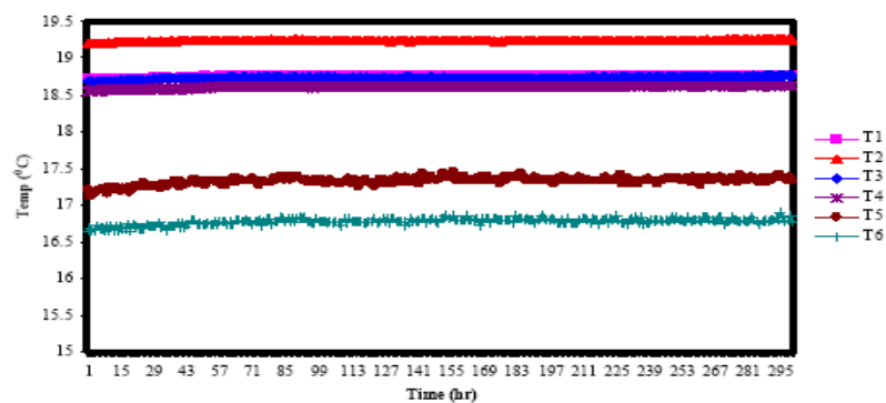
Figure 17. Variation of temperatures for heat exchanger for two weeks
