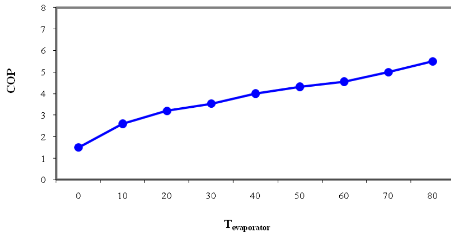
Figure 6. Heat pump performance vs evaporation temperature
