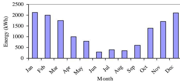
Figure 22. Monthly heating energy demands
