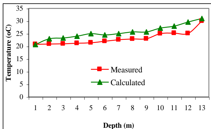
Figure 12. Comparison of calculations and experiments for unsaturated soil without groundwater flow (US)
