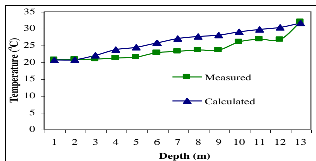
Figure 11. Comparison of calculations and experiments for saturated soil without groundwater flow (SS)
