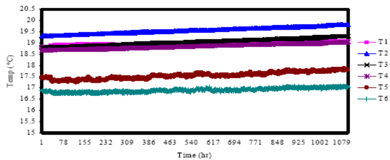
Figure 18. Variation of temperatures for heat exchanger for 45 days
