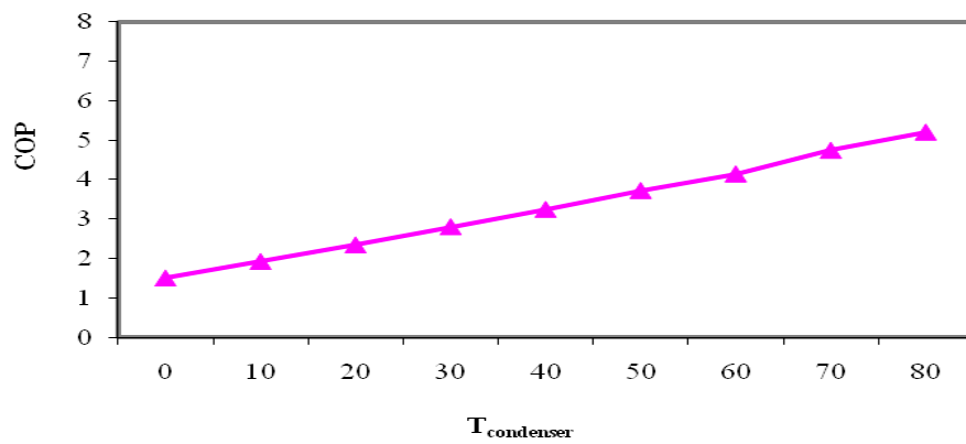
Figure 7. Heat pump performance vs condensation temperature
